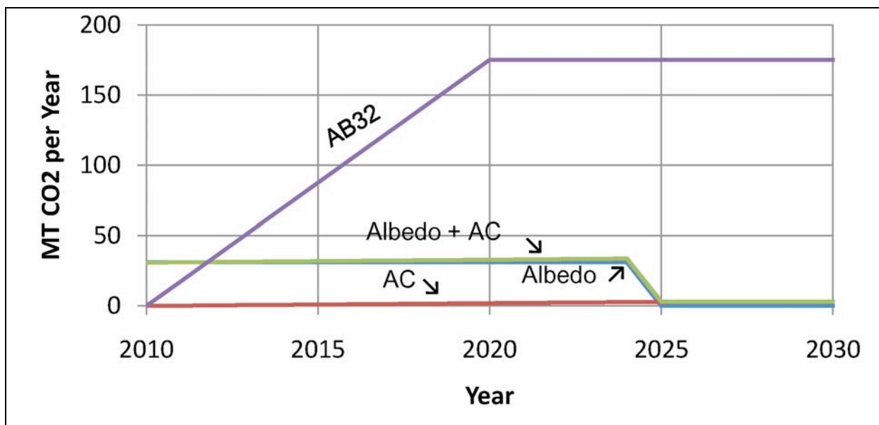
Figure 1. Comparison of CO2 saving from AB32 and offset by cool urban surfaces (roofs + pavements replaced during a 15-year program). The ‘albedo’ line is the equivalent CO2 offset (31 Mt CO2/year for 15 years). The lowest line, labeled “AC”, reaching only 3 MTCO2/yr in 2025 is the savings from avoided electricity from reduced cooling load from cool roofs. While AC savings is a lucrative measure, it is 10 times smaller than the new albedo consideration.
